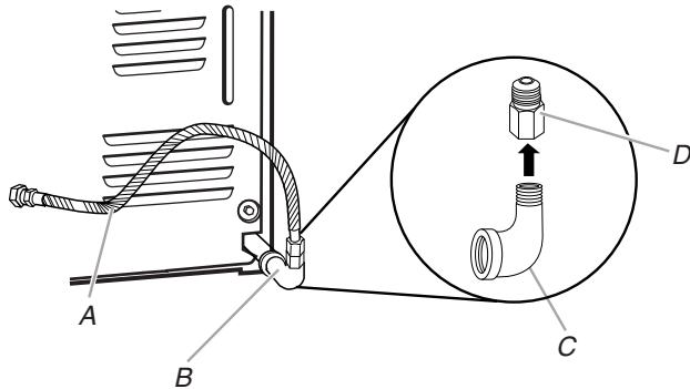
A. \frac{3}{8} " flexible gas connector B. \frac{3}{8} " dryer pipe C. \frac{3}{8} " to \frac{1}{2} " pipe elbow D. \frac{1}{2} " pipe-to-flare adapter fitting
